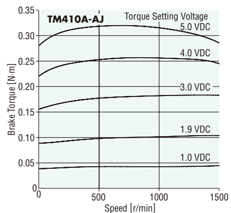
Fig. 1 Example of Speed – Brake Torque Characteristics with Reverse-Phase Brake (Reference values)
